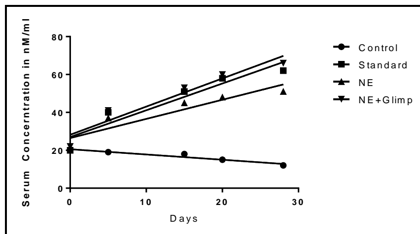
Figure 1: Effect of sub acute pretreatment of NE and Glimepiride on total antioxidant status of STZ-induced diabetic rats
