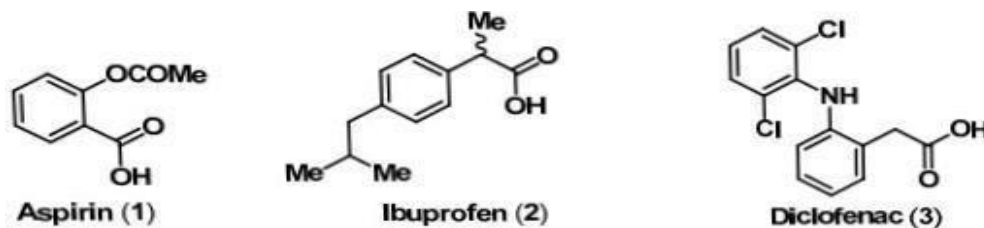
Figure 2: Chemical structures of some non- selective and selective COX inhibit
